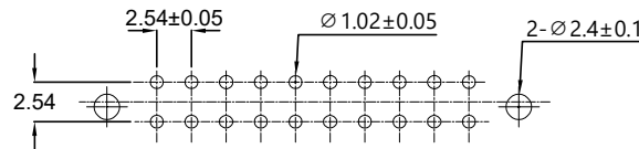
P. C. B LAYOUT
