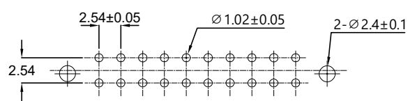
P. C. B LAYOUT
