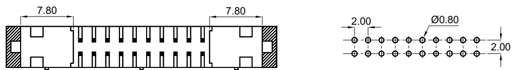
P. C. B LAYOUT
