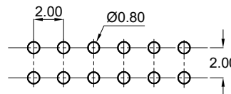
P. C. B LAYOUT
