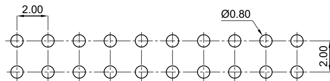
Recommended PCB Board Layout
