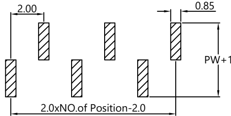
TYPE B PCB LAOUT
