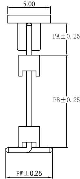
TYPE B PCB LAOUT
