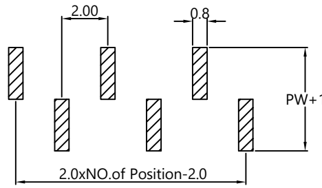
TYPE A PCB LAOUT
