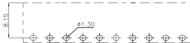
PCB LAYOUT
