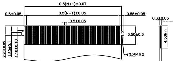
APPLICABLE FPC (+LOCK)
