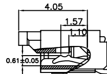
SECTION A-A (2:1)
