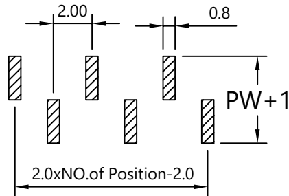
TYPE A PCB LAOUT
