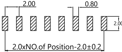
PCB LAYOUT
