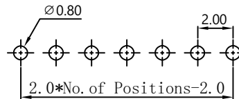
PCB LAYOUT
