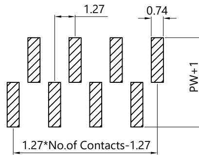
TYPE B PCB LAYOUT
