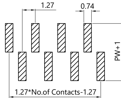
TYPE A PCB LAYOUT
