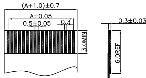
APPLICABLE FPC
