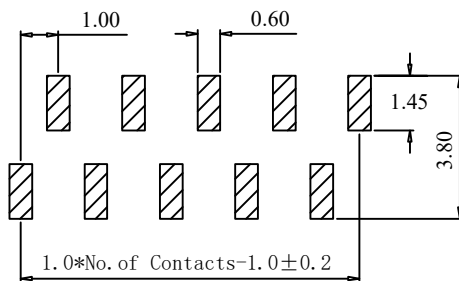
TYPE B PCB LAYOUT
