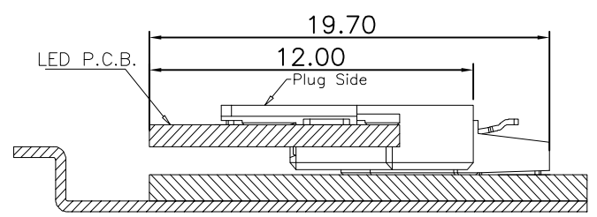
Mating Condition
