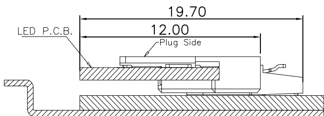
Mating Condition
