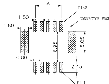
Recommended P.C.B. Layout Total tolerance: ±0.05mm
