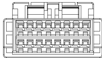
2x6-2x9P
